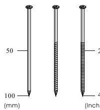
Smooth Shank Screw Shank Ring Shank Dia. 2.87-3.76mm 21 Degree Round Head
