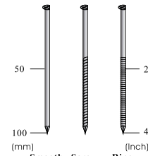
Smooth Shank Screw Shank Ring Shank Dia. 2.87-3.76mm 28 Degree & 34 Degree Clipped Head
